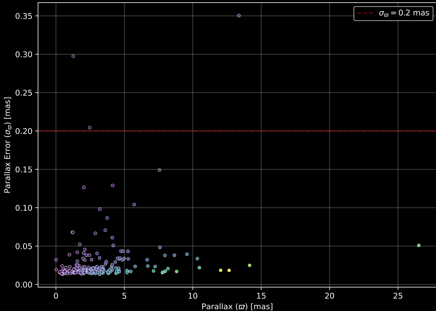
APOGEE DR17 Field: [K2_C3_057-51_btx] Parallax Quality (n= 206)
