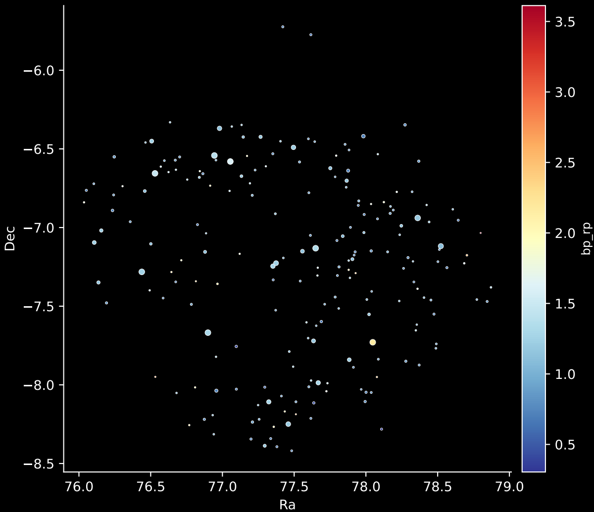
APOGEE DR17 Field: [K2_C3_057-51_btx] Stars: 206
