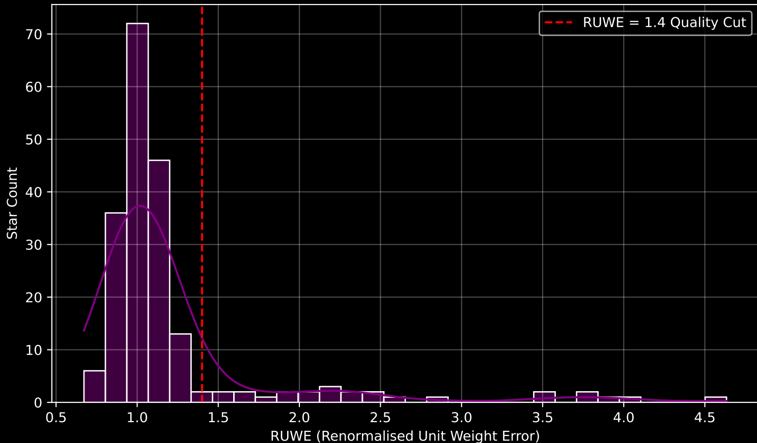
GAPOGEE DR17 Field [K2_C3_057-51_btx] RUWE Distribution (n= 200)
