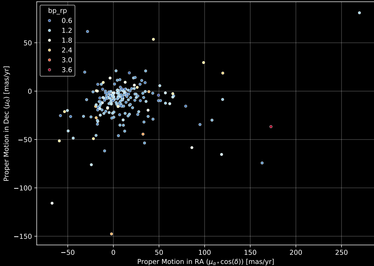
APOGEE DR17 Field: [K2_C3_057-51_btx] Proper Motion Diagram (n= 206)
