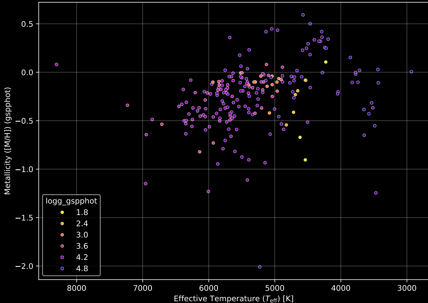
APOGEE DR17 Field: [K2_C3_057-51_btx] Stellar Population Parameters (n= 206)
