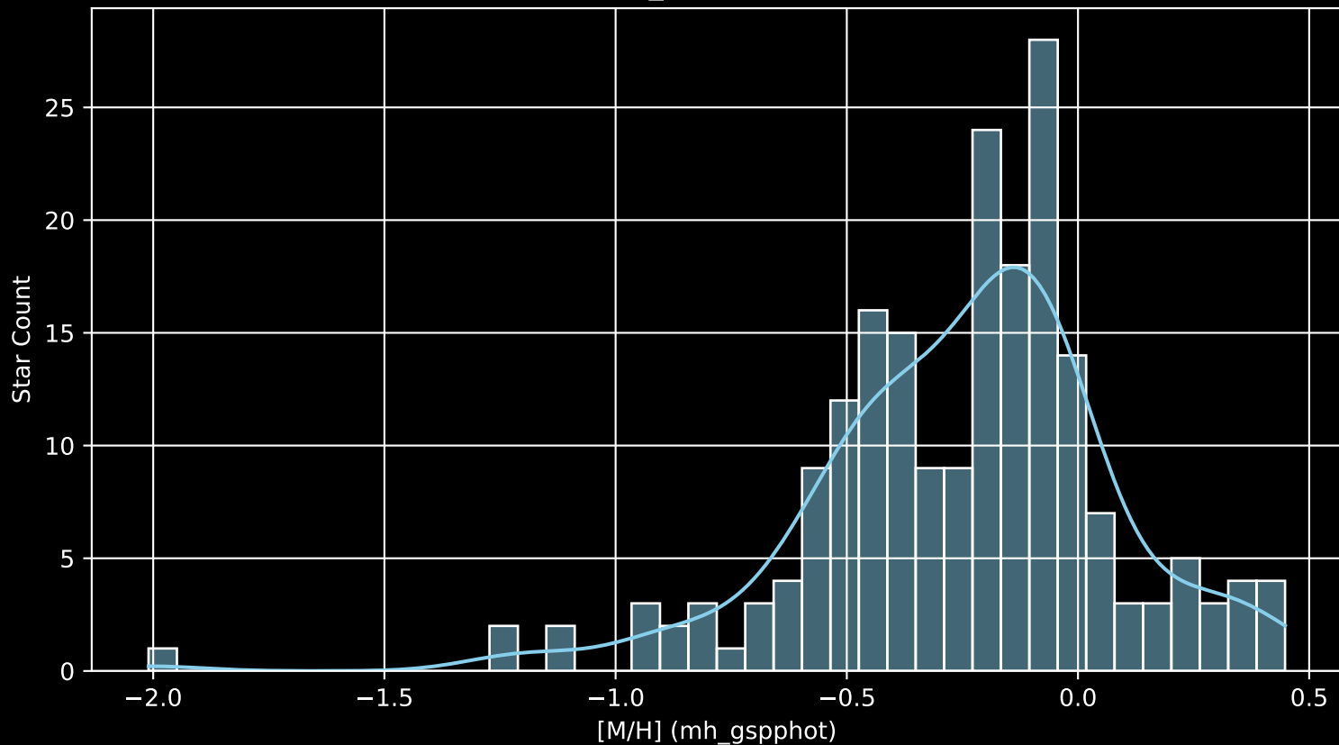
APOGEE DR17 Field: [K2_C3_057-51_btx [M/H] (mh_gspphot) (n= 204)
