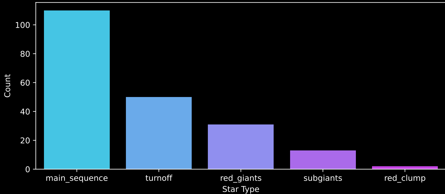
APOGEE DR17 Field: [K2_C3_057-51_btx] Count plot of Star Type
